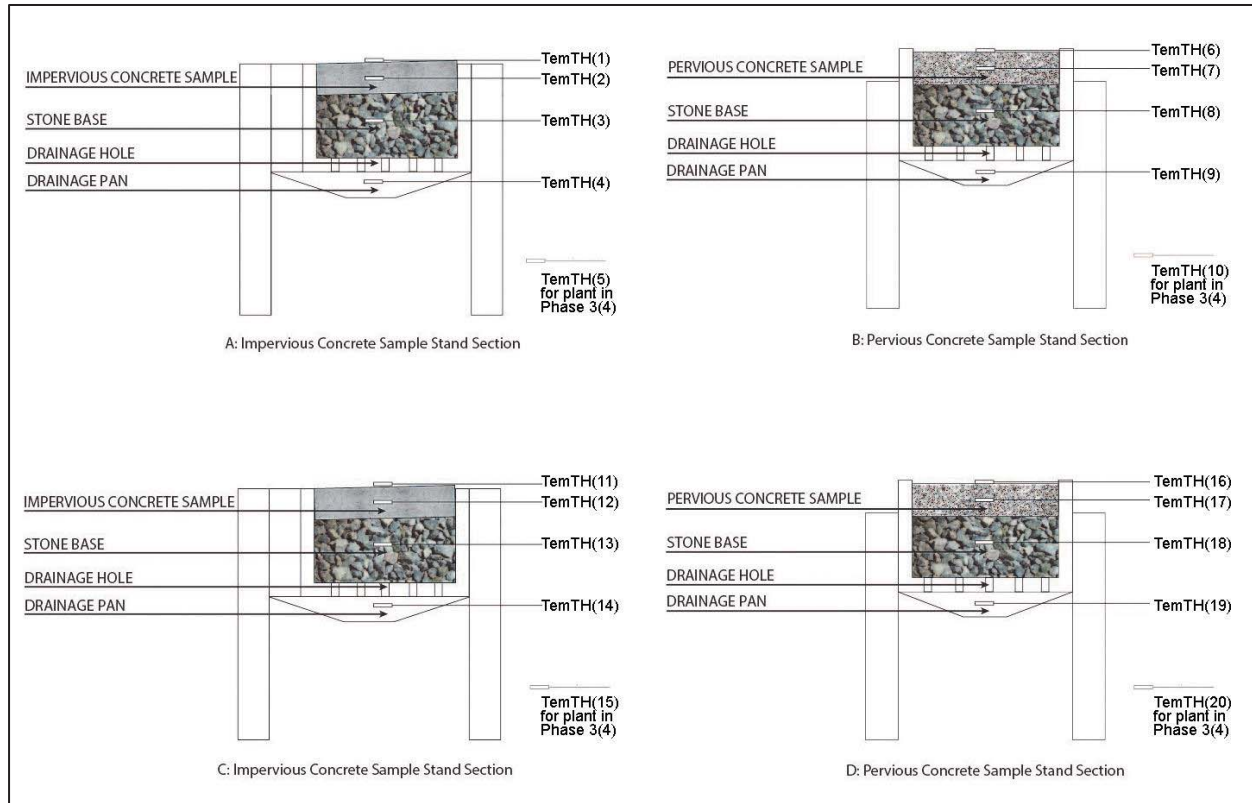
Figure 2. Phase1 samples and probes layout diagram (Figure by the authors)
