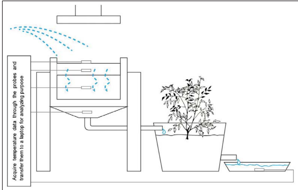
Figure 3. Phase 3 and 4 test setup and water flow diagram (Figure by the authors)
